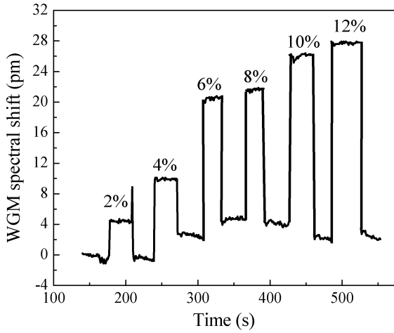
Fig. 7. Sensorgram when various concentrations of ethanol are pumped through the LCORR. Red shifts in the WGM spectral position indicate the moment when the ethanol solution entered the LCORR.
