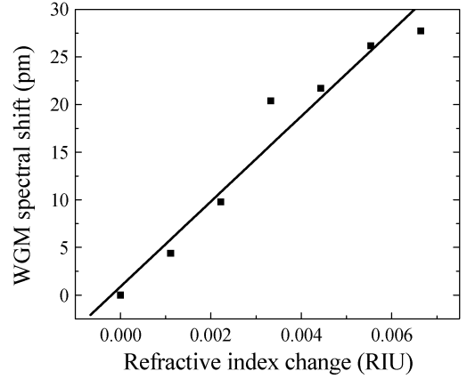
Fig. 8. WGM spectral shift versus change in refractive index for the LCORR sensor. The slope is 4.5 nm/RIU.
