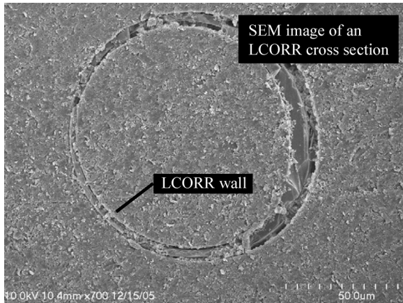
Fig. 10. SEM image of the cross-section of the LCORR. To obtain this image, the LCORR was broken at the sensing region, then covered in a UV-curable glue, and then polished at the cross-section.
