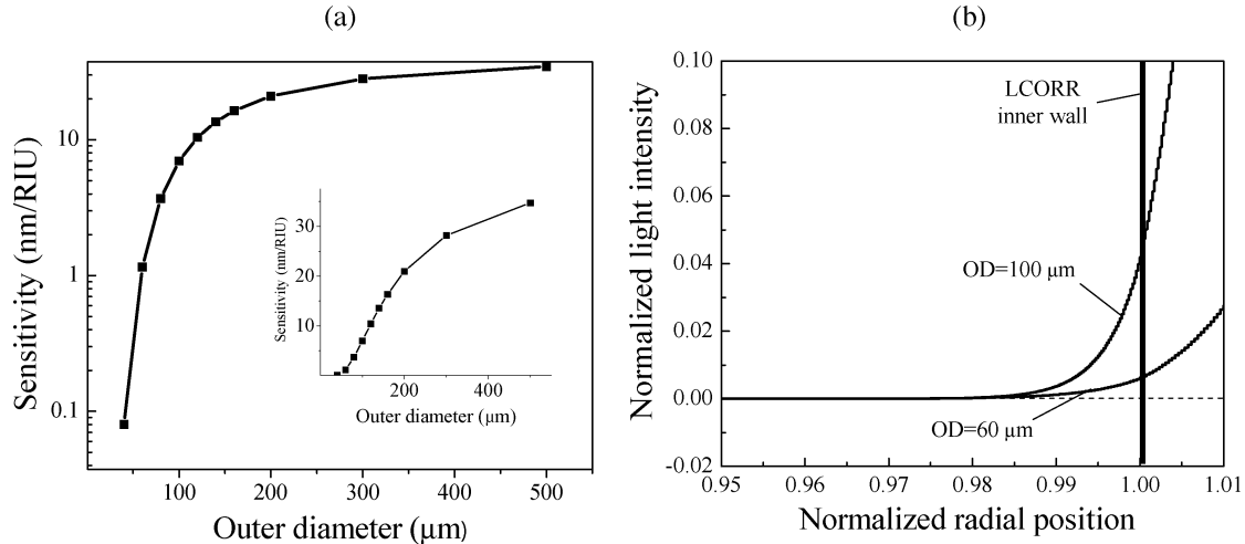
Fig. 12. (a) Calculated LCORR sensitivity dependence on the diameter; the wall thickness is held constant at 4 \mu\text{m} . The second radial TM mode is used. (b) Comparison of the evanescent intensities at the interior surface for LCORRs with diameters of 60 \mu\text{m} and 100 \mu\text{m} .
