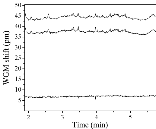
Fig. 13. Subtracting the signal produced by the reference channel from that produced by the sensing channel results in a very low noise signal.
