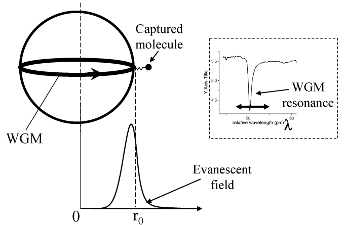
Fig. 1. Evanescent field interacts with matter near the surface of the sphere, and thus, the WGM spectral position shifts when the bulk refractive index of the solution change or when molecules bind at the surface.
