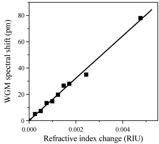
Fig. 9. WGM spectral shift versus change in refractive index when methanol is added. The slope is 16.1 nm/RIU.
