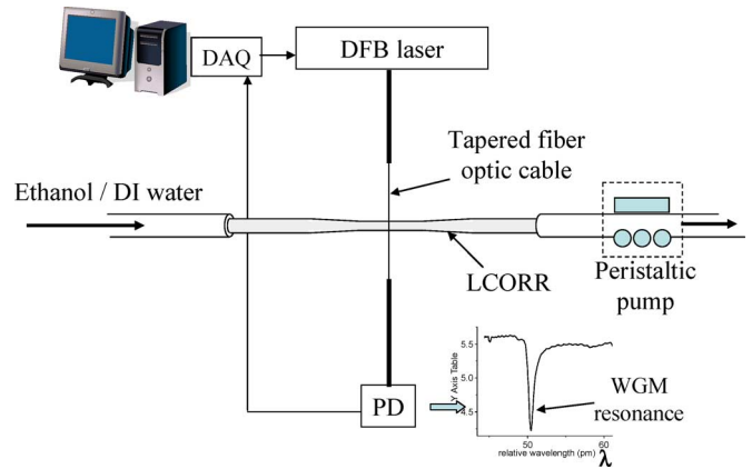
Fig. 5. Experimental setup for the LCORR sensor system.
