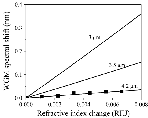
Fig. 11. Calculation of the sensitivity for LCORR wall thicknesses of 3 \mu\text{m} , 3.5 \mu\text{m} , and 4.2 \mu\text{m} . The second radial TM mode is used. Experimental data (■) is shown for comparison with the calculation using a 4.2- \mu\text{m} wall thickness.
