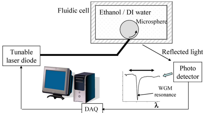
Fig. 4. Experimental setup for the microsphere resonator sensor system.
