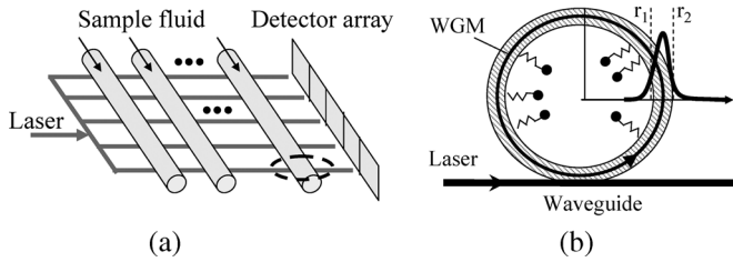
Fig. 3. (a) Two-dimensional arrangement of LCORRs. Each LCORR is in contact with several waveguides or fiber tapers, and each LCORR is patterned with the desired surface functionalization at each waveguide/taper connection point. (b) Cross section of a single LCORR, as circled in (a).
